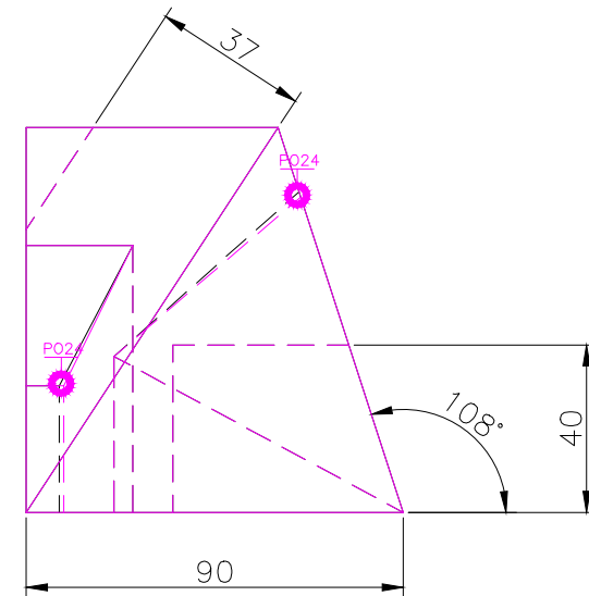
RIGHT SCALE 1/2
