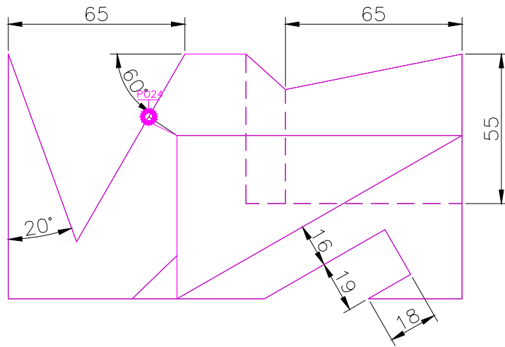
TOP SCALE 1/2
