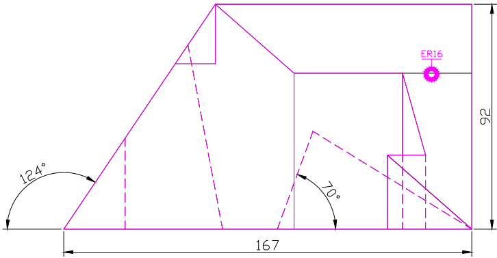
FRONT SCALE 1/2
