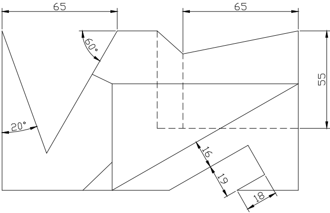
TOP SCALE 1/2
