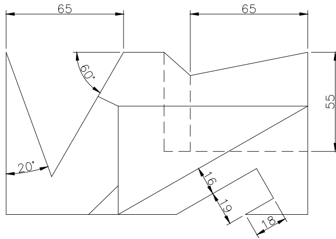
TOP SCALE 1/2
