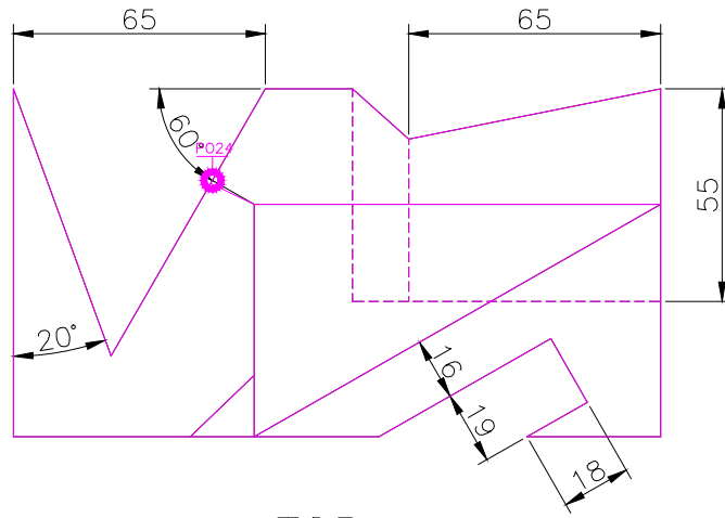
TOP SCALE 1/2
