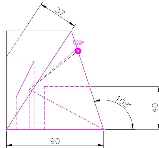
RIGHT SCALE 1/2
