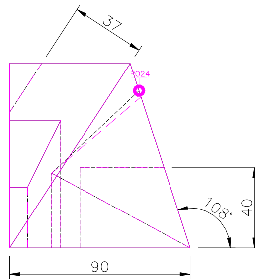
RIGHT SCALE 1/2
