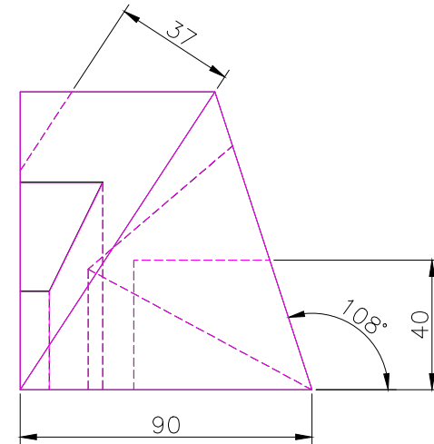
RIGHT SCALE 1/2
