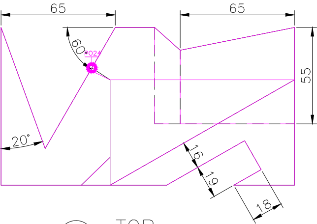
TOP SCALE 1/2
