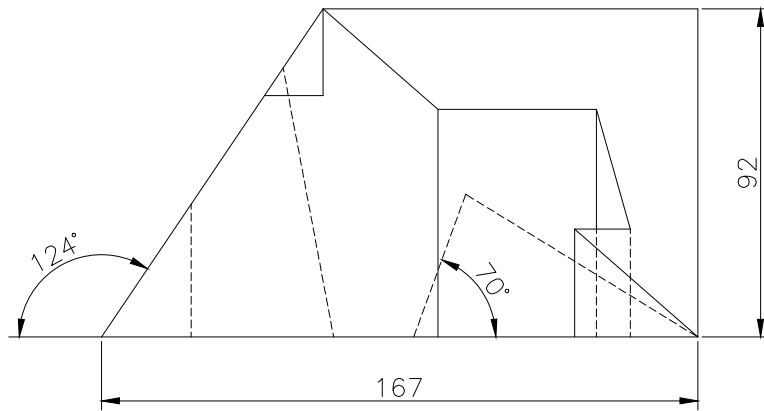
FRONT SCALE 1/2
