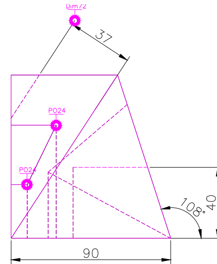
RIGHT SCALE 1/2
