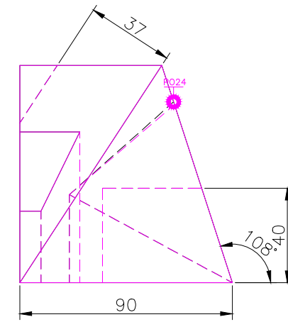
RIGHT SCALE 1/2
