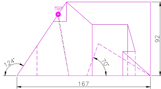
FRONT SCALE 1/2
