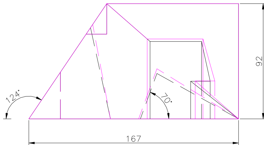
FRONT SCALE 1/2
