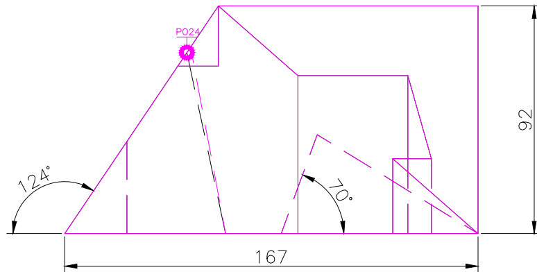
FRONT SCALE 1/2
