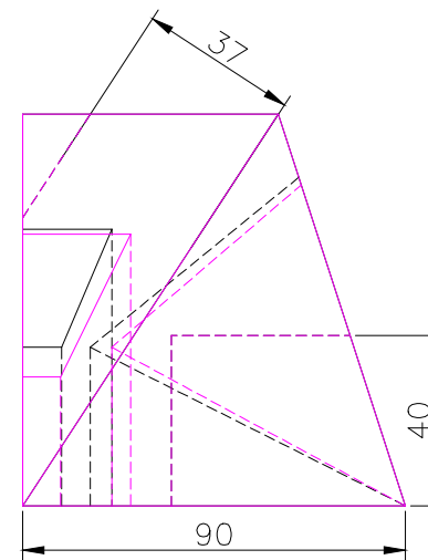
RIGHT SCALE 1/2
