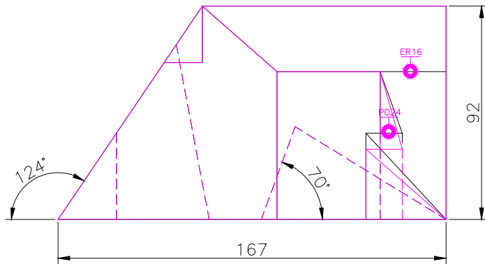
FRONT SCALE 1/2
