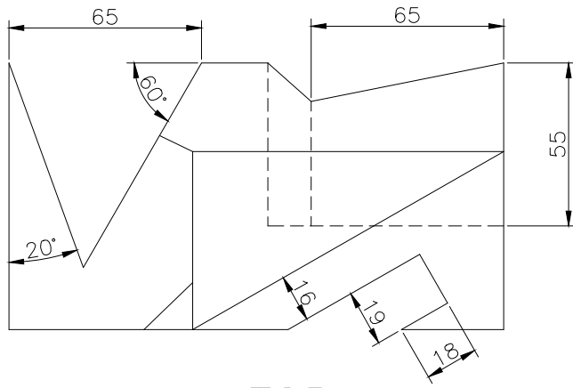
TOP SCALE 1/2
