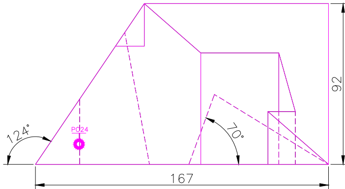
FRONT SCALE 1/2
