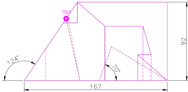
FRONT SCALE 1/2
