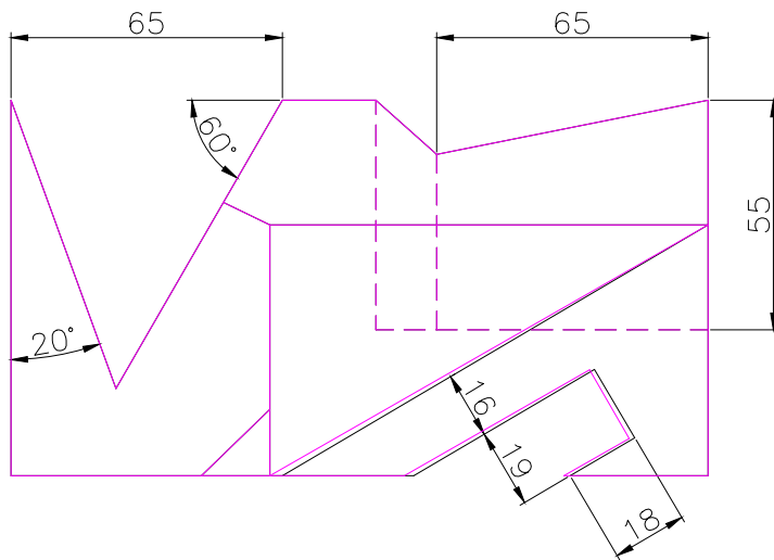
TOP SCALE 1/2
