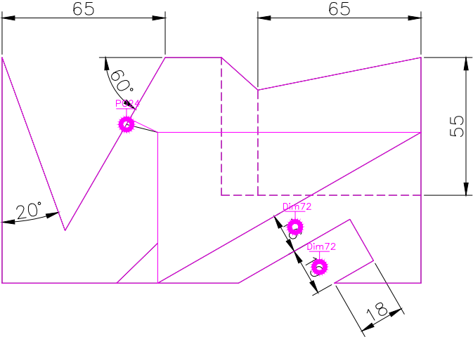
TOP SCALE 1/2
