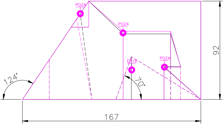
FRONT SCALE 1/2
