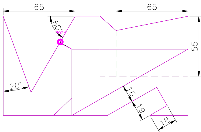
TOP SCALE 1/2
