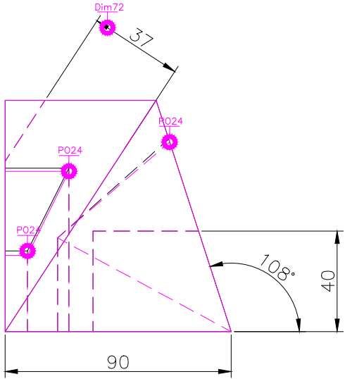
RIGHT SCALE 1/2
