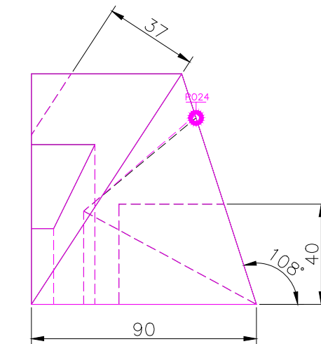
RIGHT SCALE 1/2
