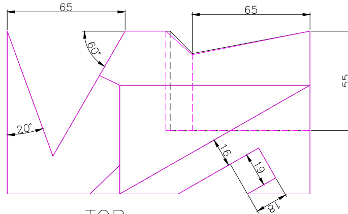
TOP SCALE 1/2
