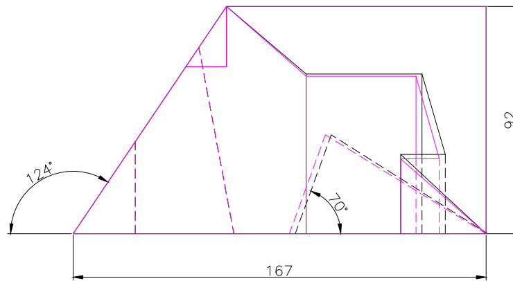
FRONT SCALE 1/2
