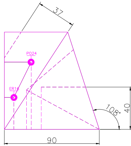
RIGHT SCALE 1/2
