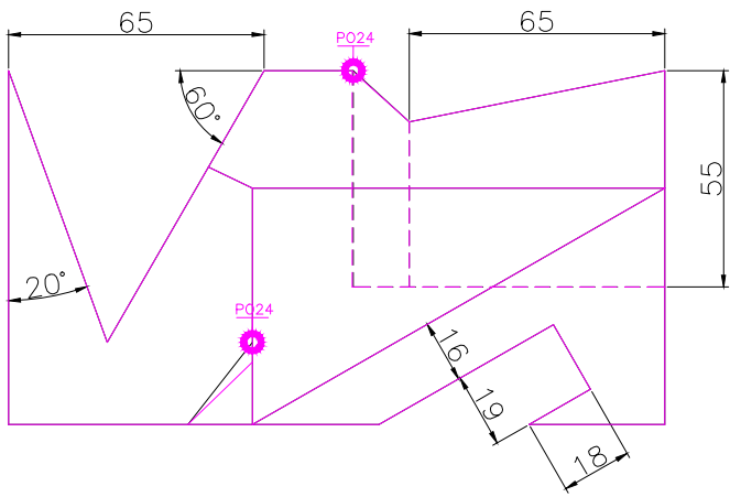
TOP SCALE 1/2
