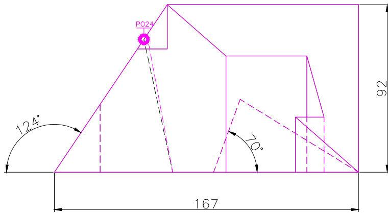
FRONT SCALE 1/2
