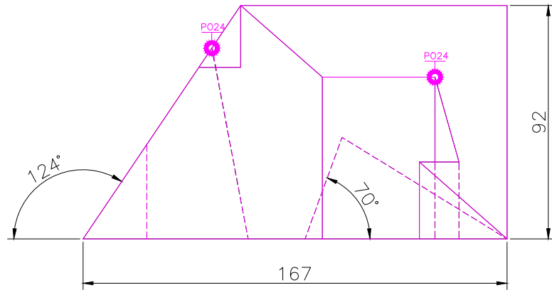
FRONT SCALE 1/2
