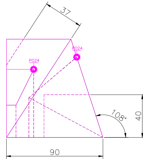
RIGHT SCALE 1/2
