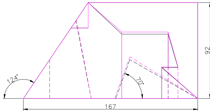
FRONT SCALE 1/2
