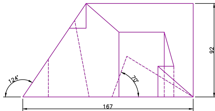
FRONT SCALE 1/2
