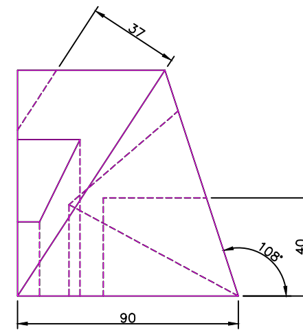
RIGHT SCALE 1/2
