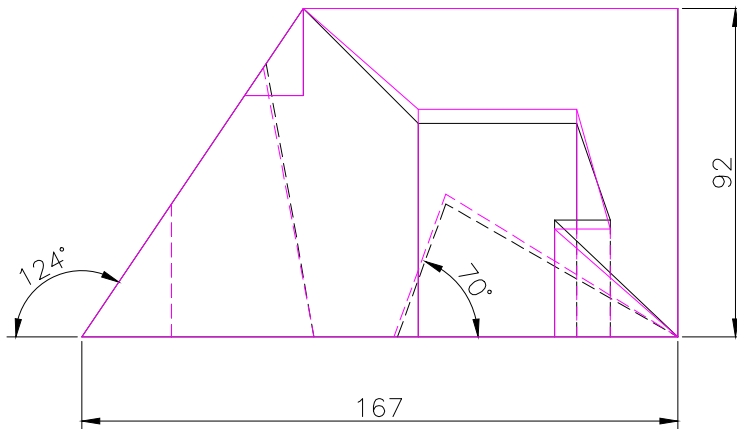
FRONT SCALE 1/2
