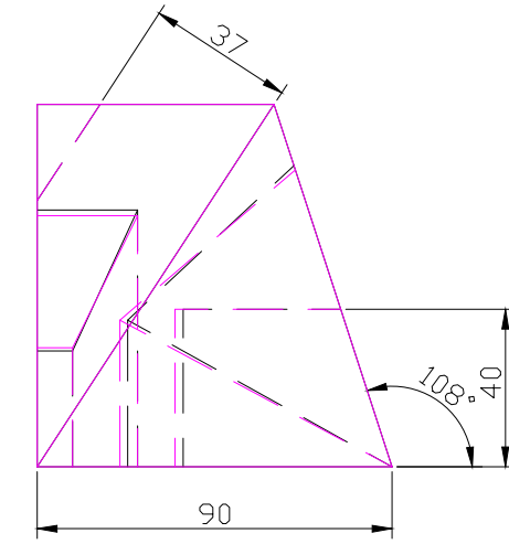
RIGHT 1/2 SCALE
