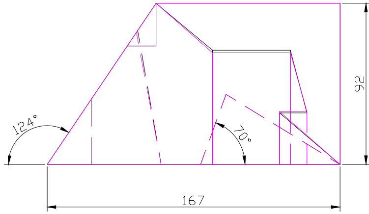
FRONT 1/2 SCALE
