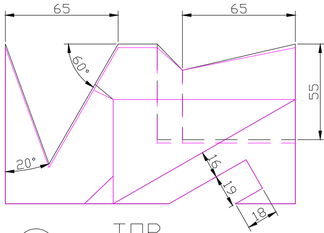
TOP 1/2 SCALE
