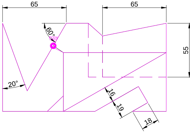
TOP SCALE 1/2
