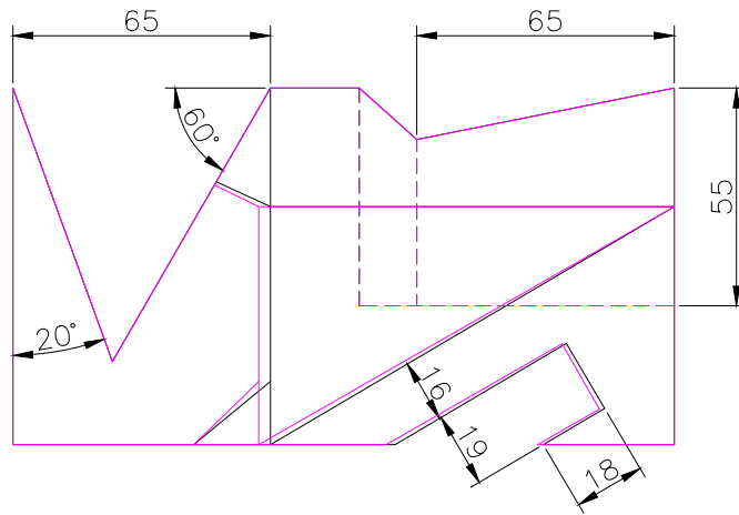
TOP SCALE 1/2
