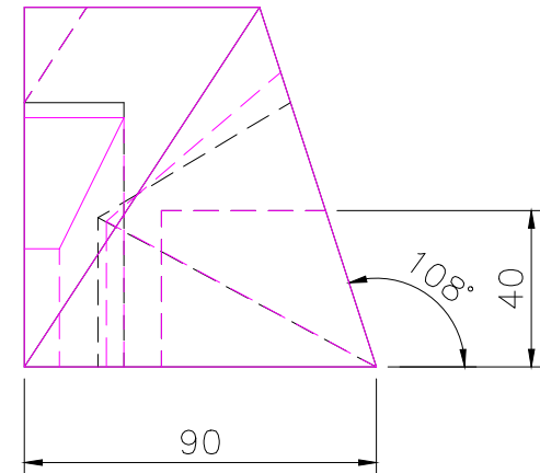
RIGHT SCALE 1/2
