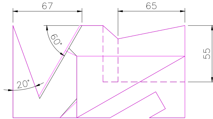
TOP SCALE 1/2
