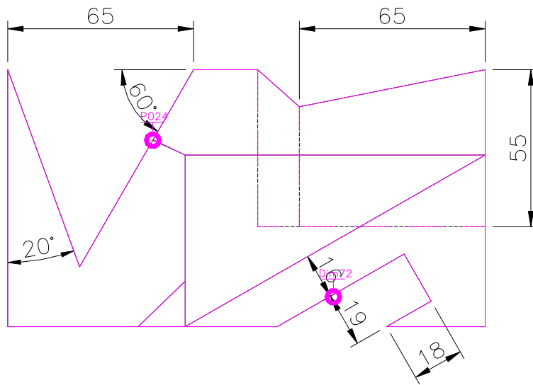
TOP SCALE 1/2
