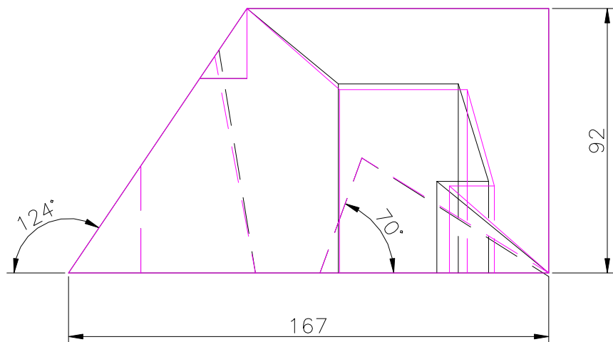
FRONT SCALE 1/2
