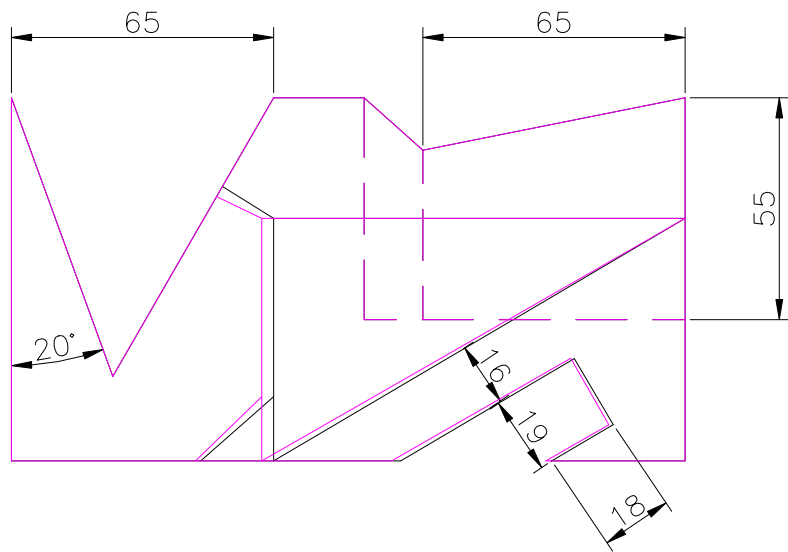
TOP SCALE 1/2
