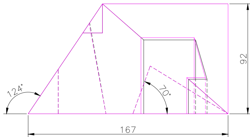
FRONT SCALE 1/2
