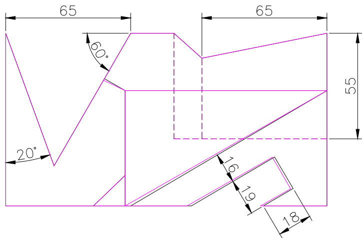
TOP SCALE 1/2
