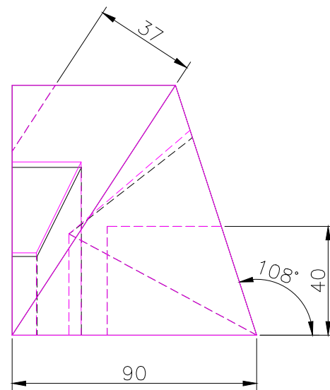
RIGHT SCALE 1/2
