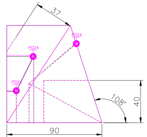
RIGHT SCALE 1/2
