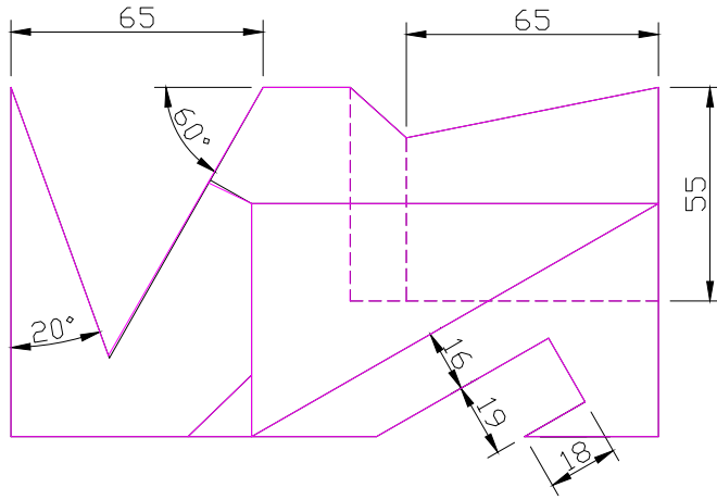
TOP SCALE 1/2
