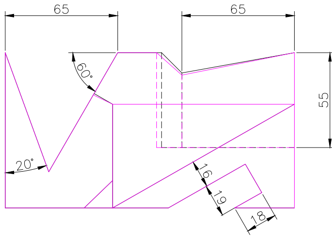
TOP SCALE 1/2
