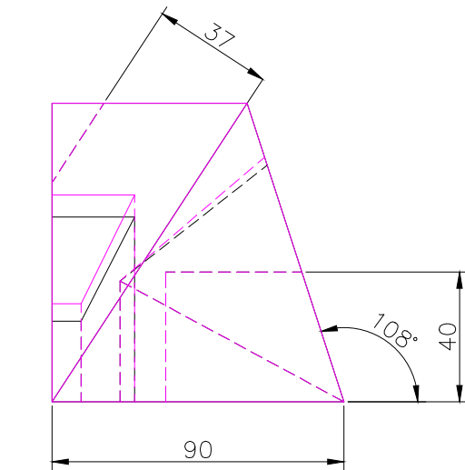
RIGHT SCALE 1/2
