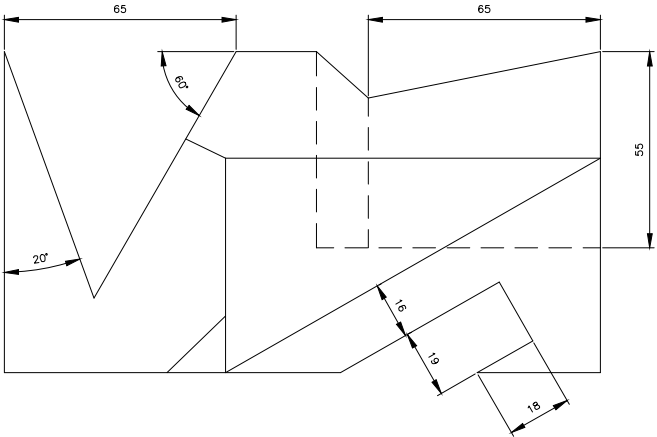
TOP SCALE 1/2
