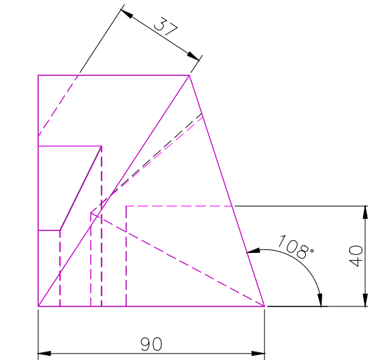
RIGHT SCALE 1/2
