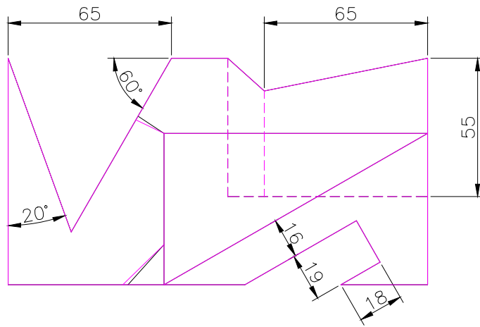
TOP SCALE 1/2
