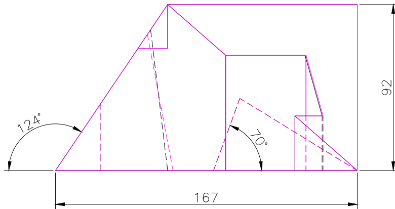
FRONT SCALE 1/2
