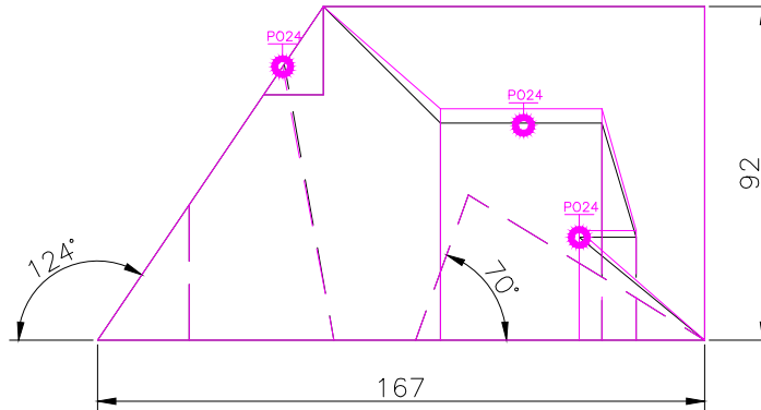
FRONT SCALE 1/2
