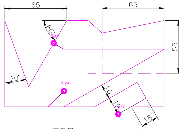
TOP SCALE 1/2
