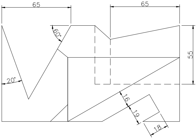
TOP SCALE 1/2
