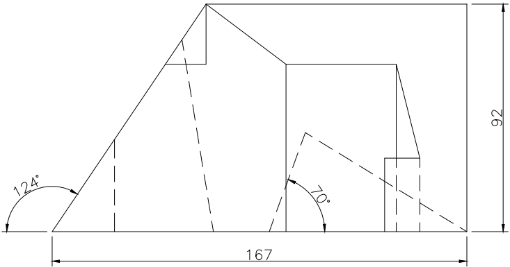
FRONT SCALE 1/2
