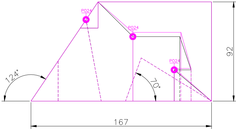
FRONT SCALE 1/2
