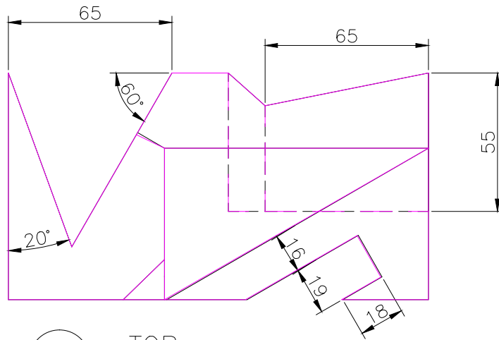
TOP SCALE 1/2
