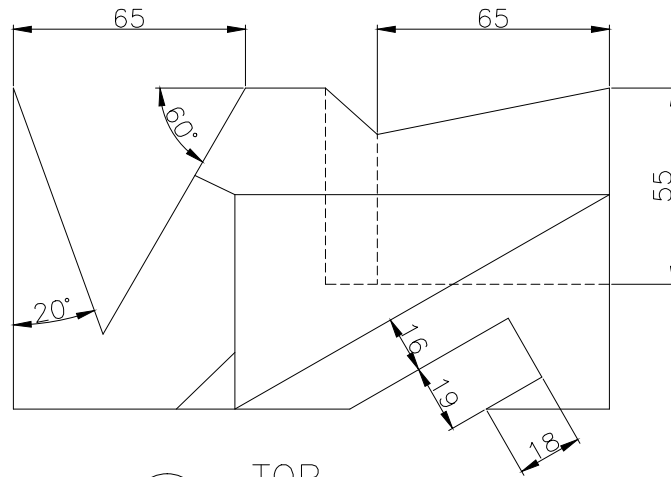
TOP SCALE 1/2
