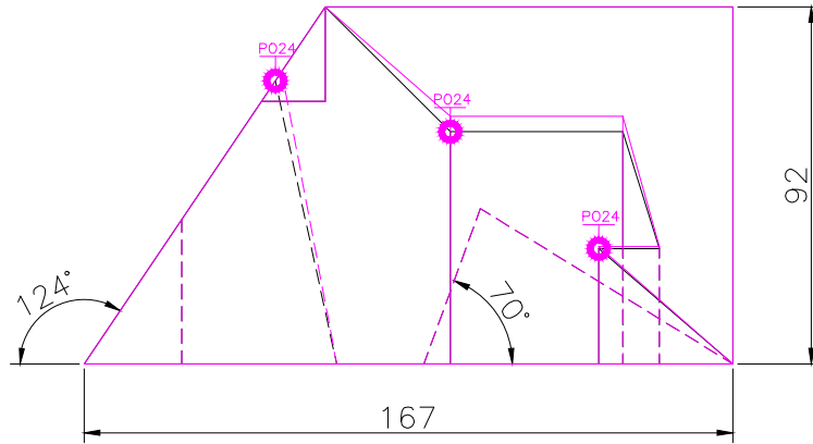
FRONT SCALE 1/2
