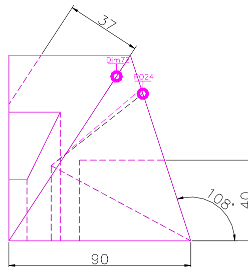
RIGHT SCALE 1/2
