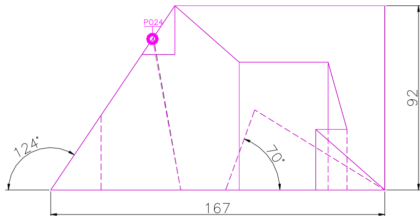
FRONT SCALE 1/2
