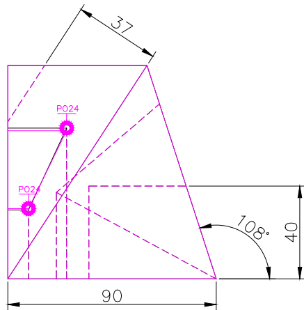
RIGHT SCALE 1/2
