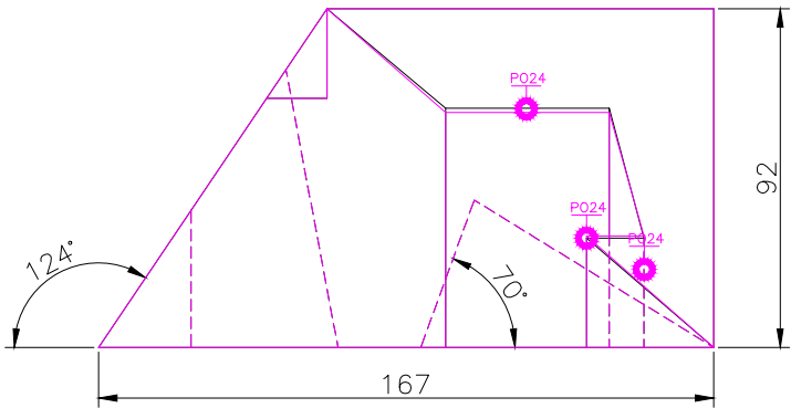
FRONT SCALE 1/2
