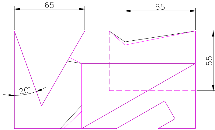
TOP SCALE 1/2
