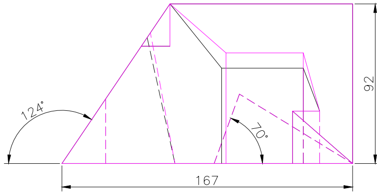
FRONT SCALE 1/2
