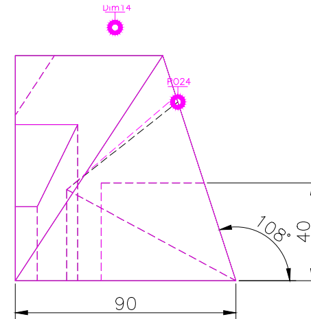
RIGHT SCALE 1/2
